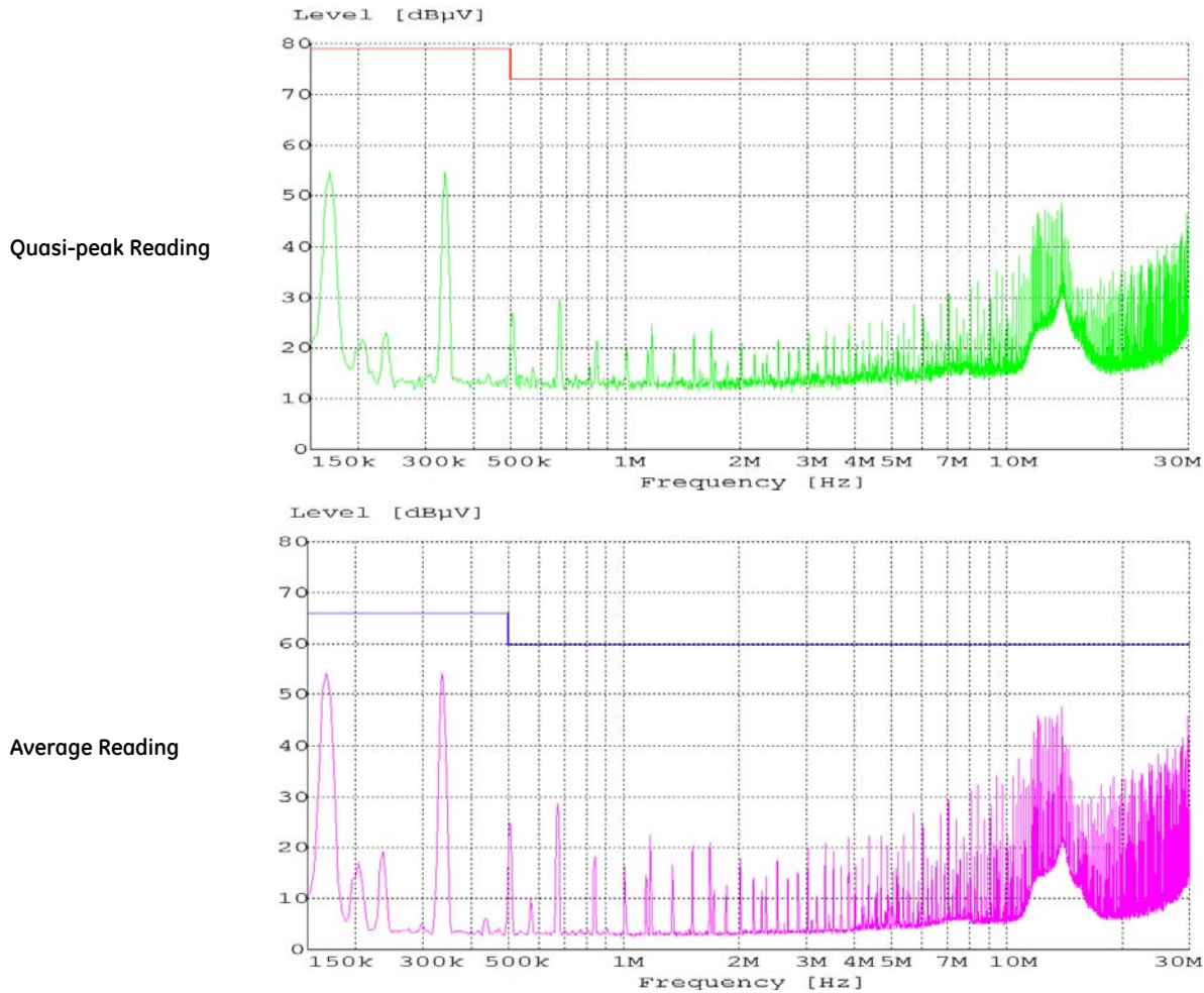
Figure 24. EMC Considerations
